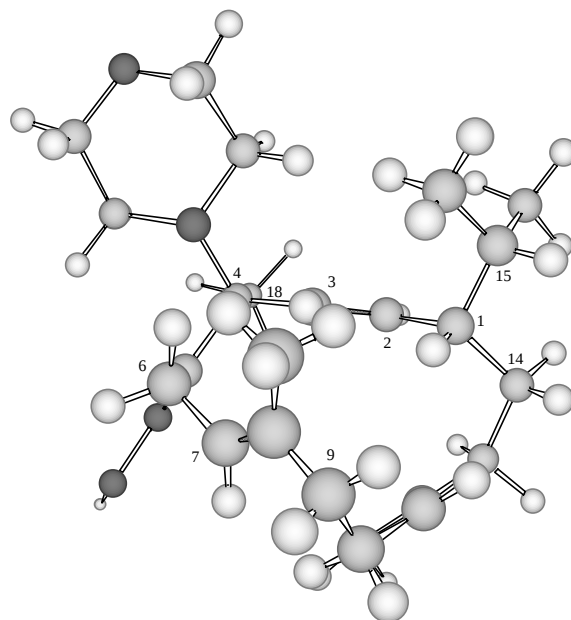
Figure 1 Molecular structure of the most stable conformation of compound 4 . The characteristic dihedral angles and calculated and experimental spin-spin coupling constants are as follows: H1–C1–C2–H2 +158°, ^3J_{\text{calc.}} 10.3 Hz ( ^3J_{\text{exp.}} 9.3 Hz); H1–C1–C14–H14 \alpha –160°, ^3J_{\text{calc.}} 11.5 Hz ( ^3J_{\text{exp.}} 9.3 Hz); H1–C1–C14–H14 \beta –49°, ^3J_{\text{calc.}} 2.3 Hz ( ^3J_{\text{exp.}} 4.3 Hz); H6 \alpha –C6–C7–H7 +63°, ^3J_{\text{calc.}} 3.4 Hz ( ^3J_{\text{exp.}} 3.0 Hz); H6 \beta –C6–C7–H7 +163°, ^3J_{\text{calc.}} 10.8 Hz ( ^3J_{\text{exp.}} 10.8 Hz); H1–C1–C15–H15 +65°, ^3J_{\text{calc.}} 3.4 Hz ( ^3J_{\text{exp.}} 4.4 Hz).
